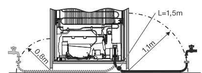
Installation possibilities to mains water KFNS 37692 iDE
